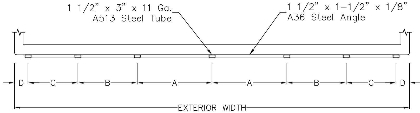
END ELEVATION VIEW
