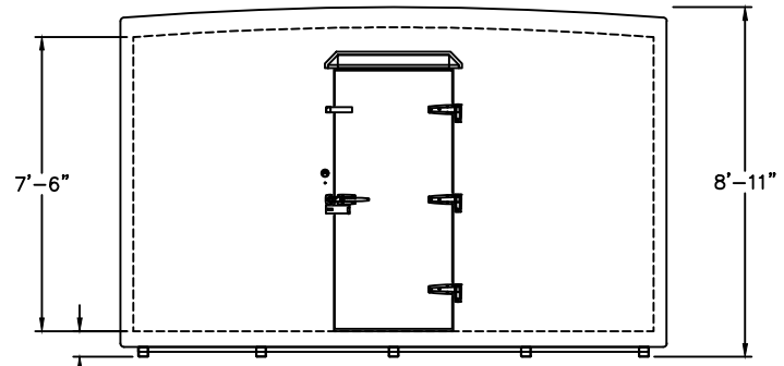
ELEVATION VIEW
