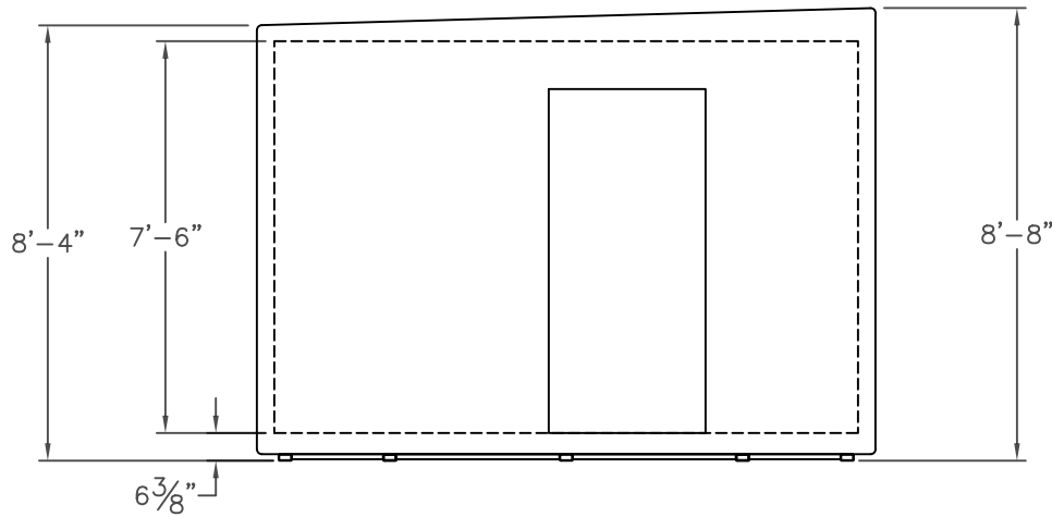
ELEVATION VIEW
