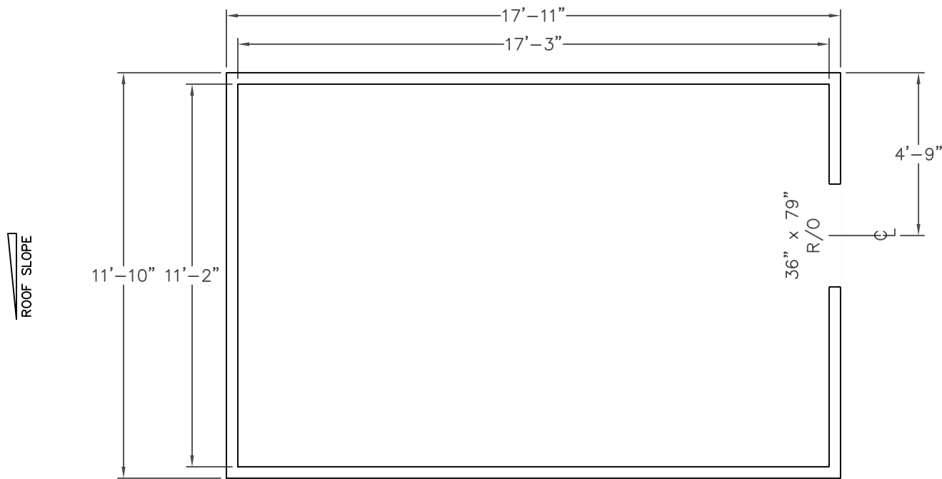
PLAN VIEW
