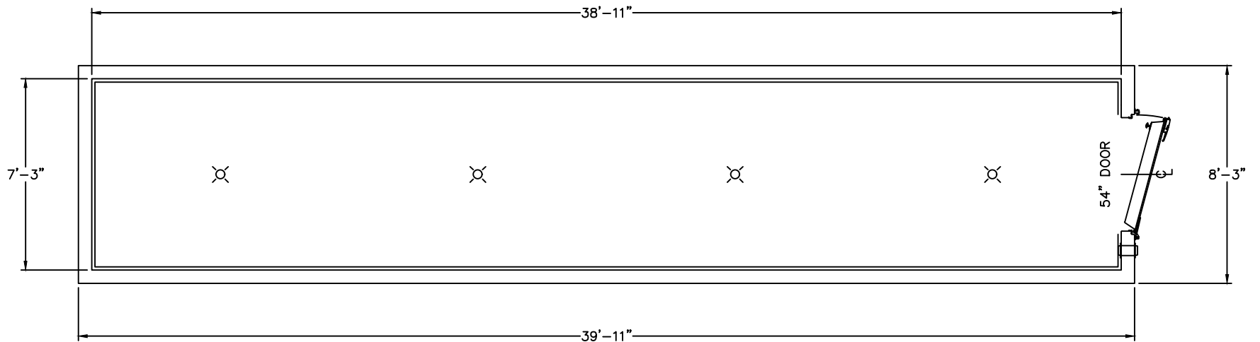
PLAN VIEW
