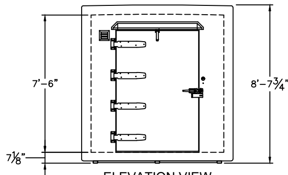
ELEVATION VIEW
