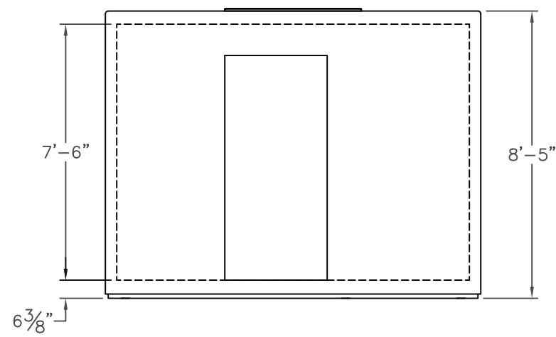
ELEVATION VIEW
