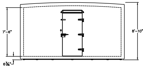
ELEVATION VIEW
