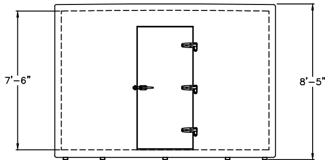
ELEVATION VIEW
