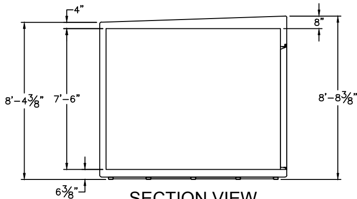
SECTION VIEW
