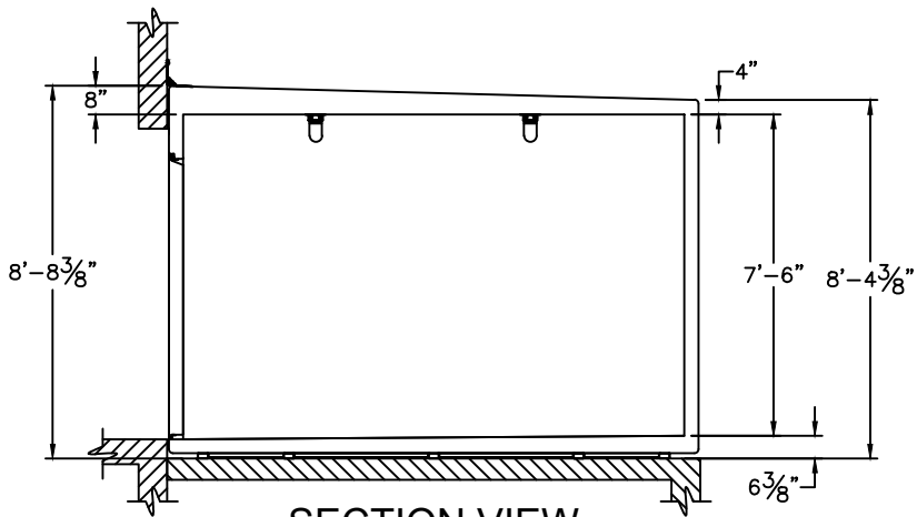
SECTION VIEW
