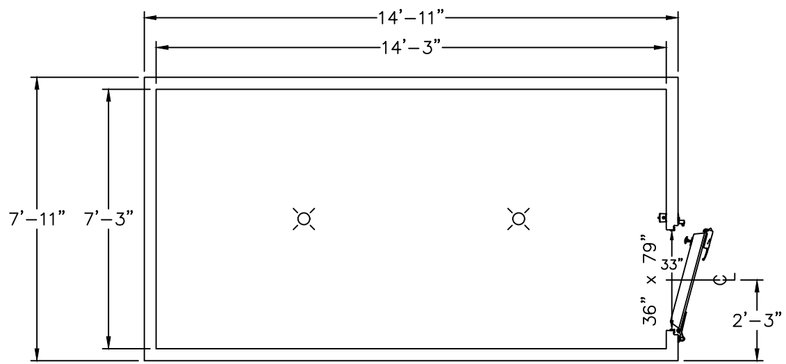
PLAN VIEW
